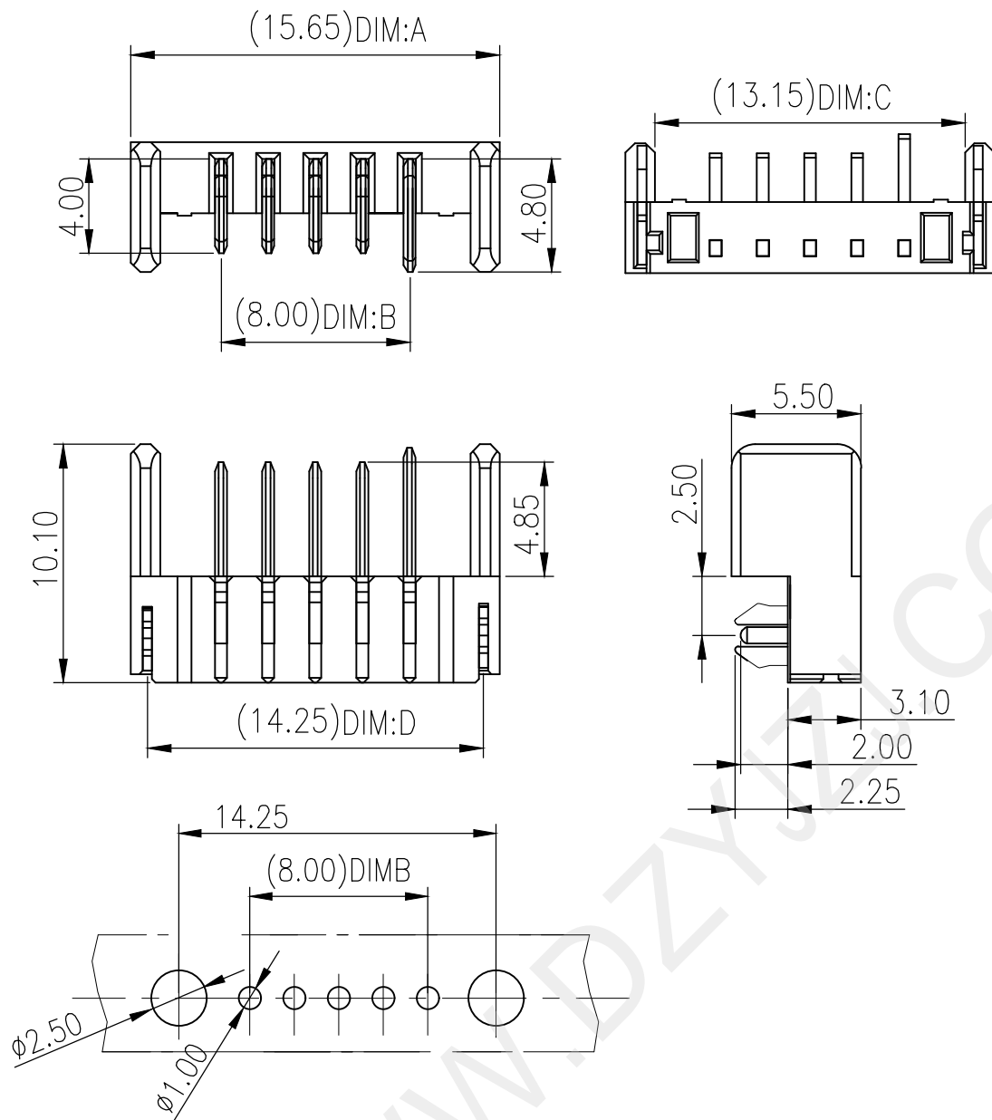
Recommended P.C.B Layout
